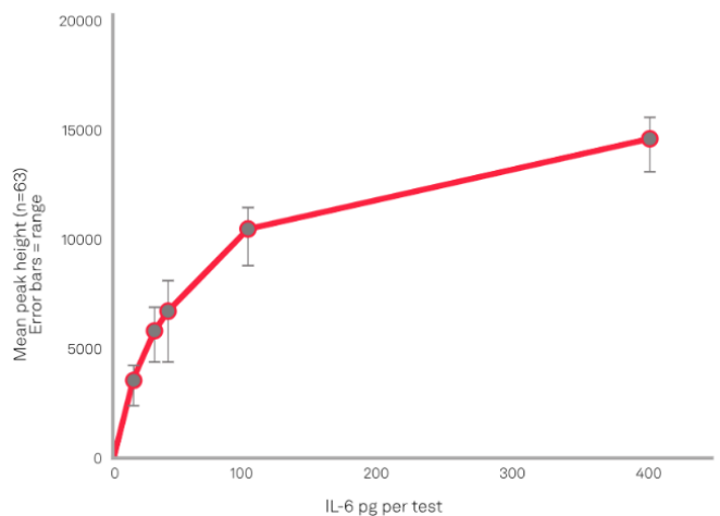
IL-6 Lateral flow - multi-day robustness study
